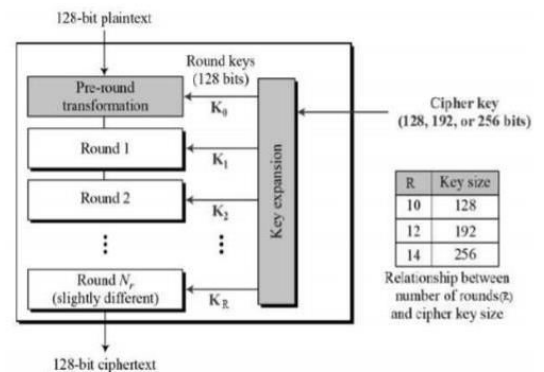
Fig-4: Encryption Process
