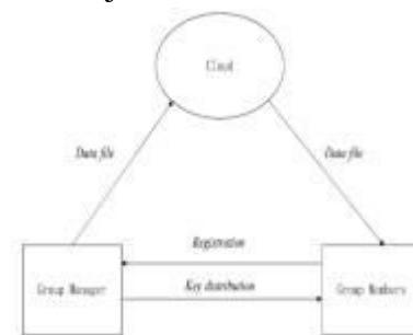
Fig 1: SYSTEM ARCHITECTURE
