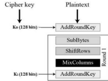
Fig -3: Operations
