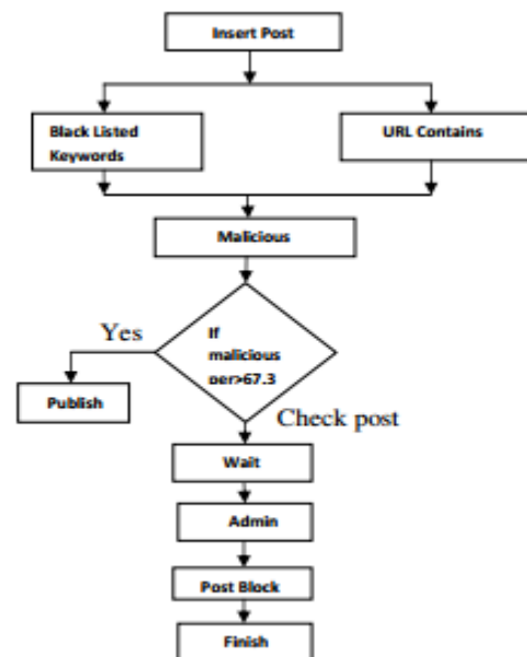
Fig 3: Proposed Methodology
