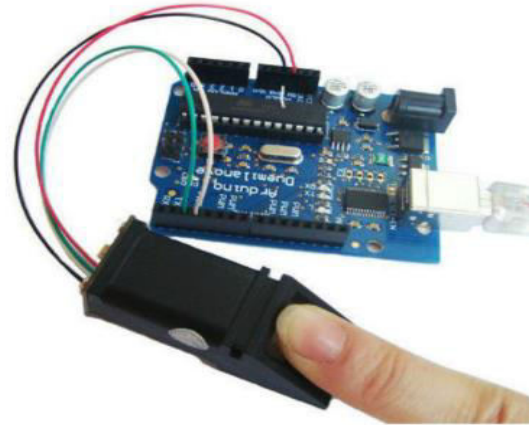
Fig.3.1. Working model.
