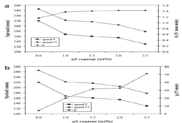
Figure 1: Influence of nS content on spread (after 0 and 15 strokes) and rheological
