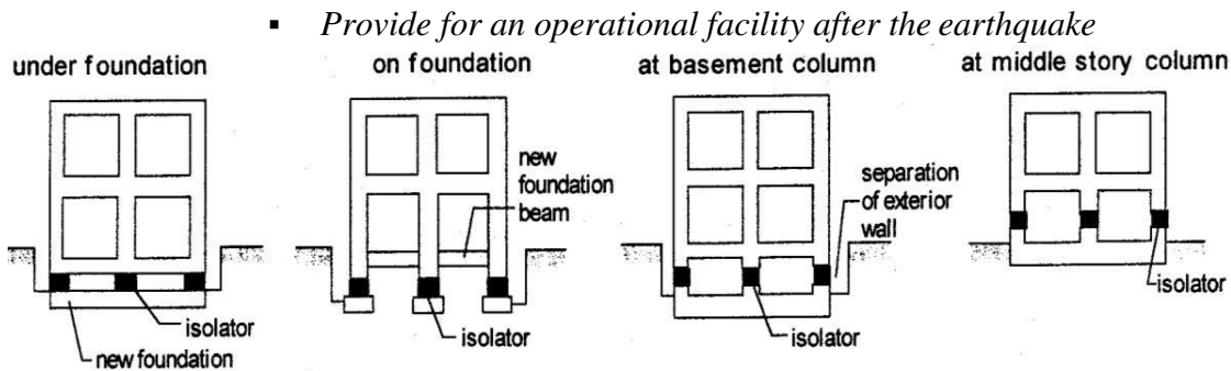
Fig.2 Isolator Components Between the Foundation and Superstructure
