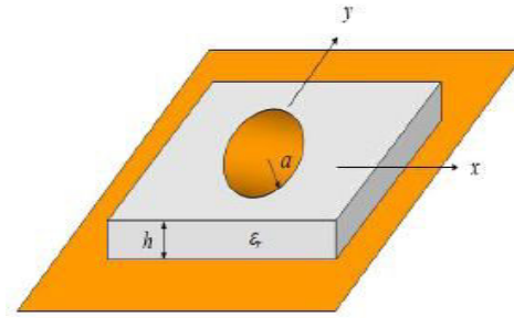
Fig.2: Circular Patch Antenna
