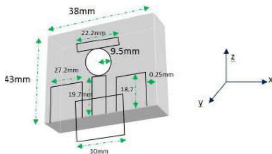
Fig.1: Antenna structure
