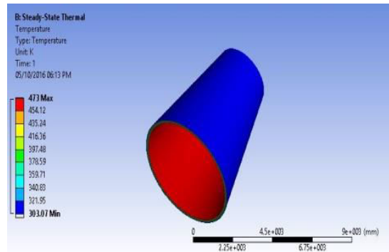
Fig 7 temperature distribution
