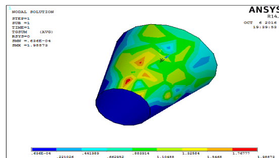
Fig 13: heat flux
