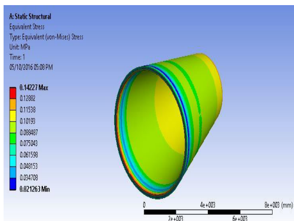
Fig 10: stress
