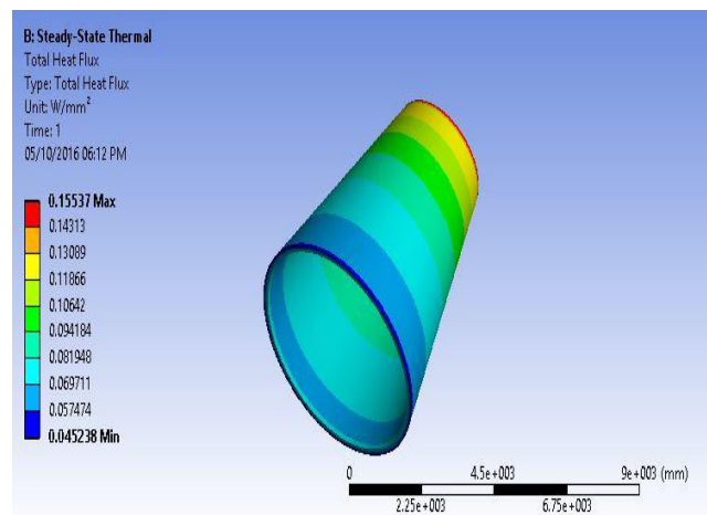
Fig 8 heat flux
