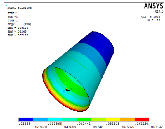
Fig 15 1: stress
