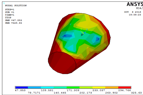
Fig 12:temperature
