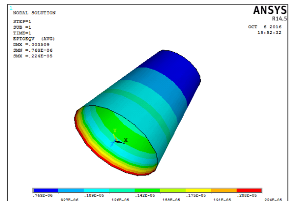
Fig16: strain
