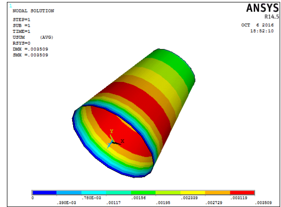
Fig14: deformation
