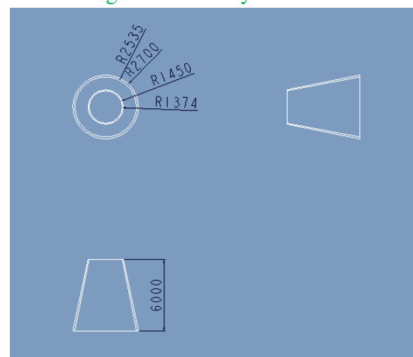
Fig 3 2D chimney model
