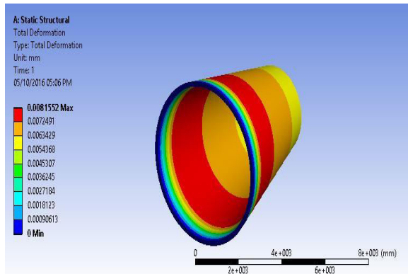
Fig 9: deformation
