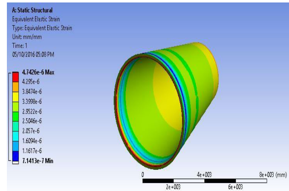
Fig 11: strain
