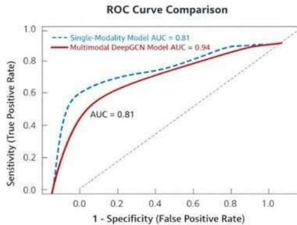
FIG 2.Roc Curve Graph
