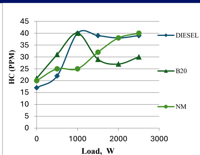
Figure 8: load vs. hydrocarbons
