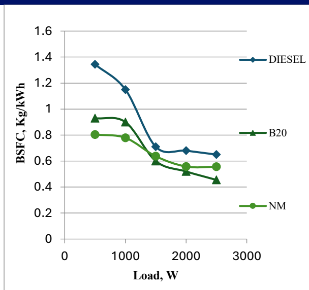
Figure 5: load vs. brake specific fuel consumption
