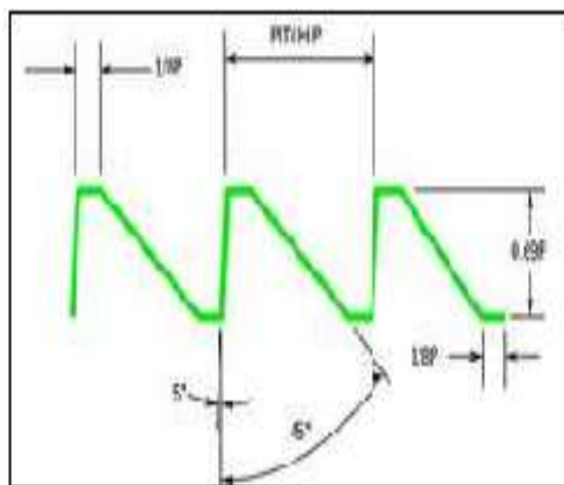
3: Profile of Buttress Thread [2] If P = Pitch of the thread, d = depth of the thread
