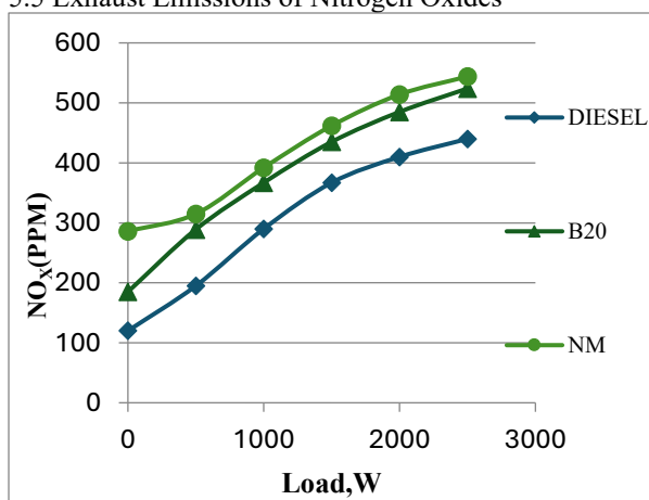
Figure 9: load vs. nitrogen oxides
