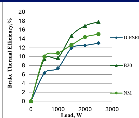
Fig 6: load vs. brake thermal efficiency
