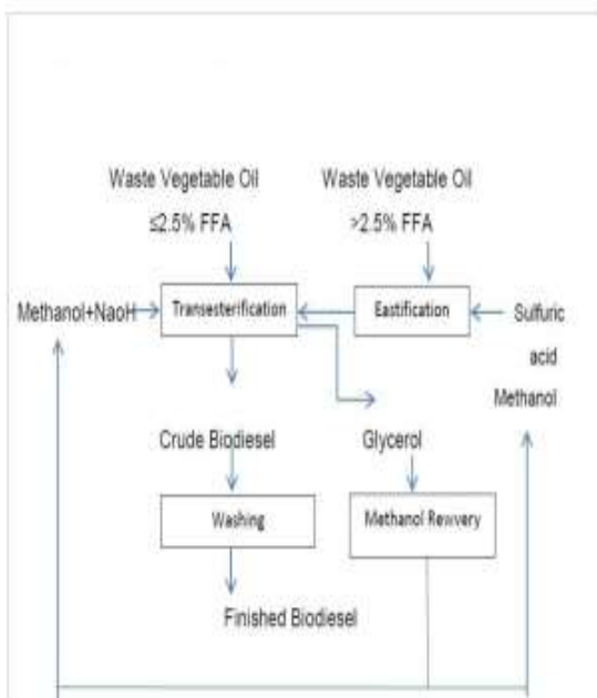
Figure 2: Process Flow for Biodiesel Process
