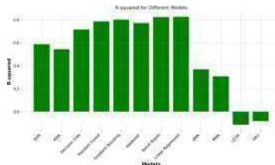
Fig 2: R2 Squared
