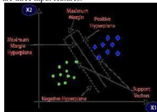
Figure 5: SVM Classifier
