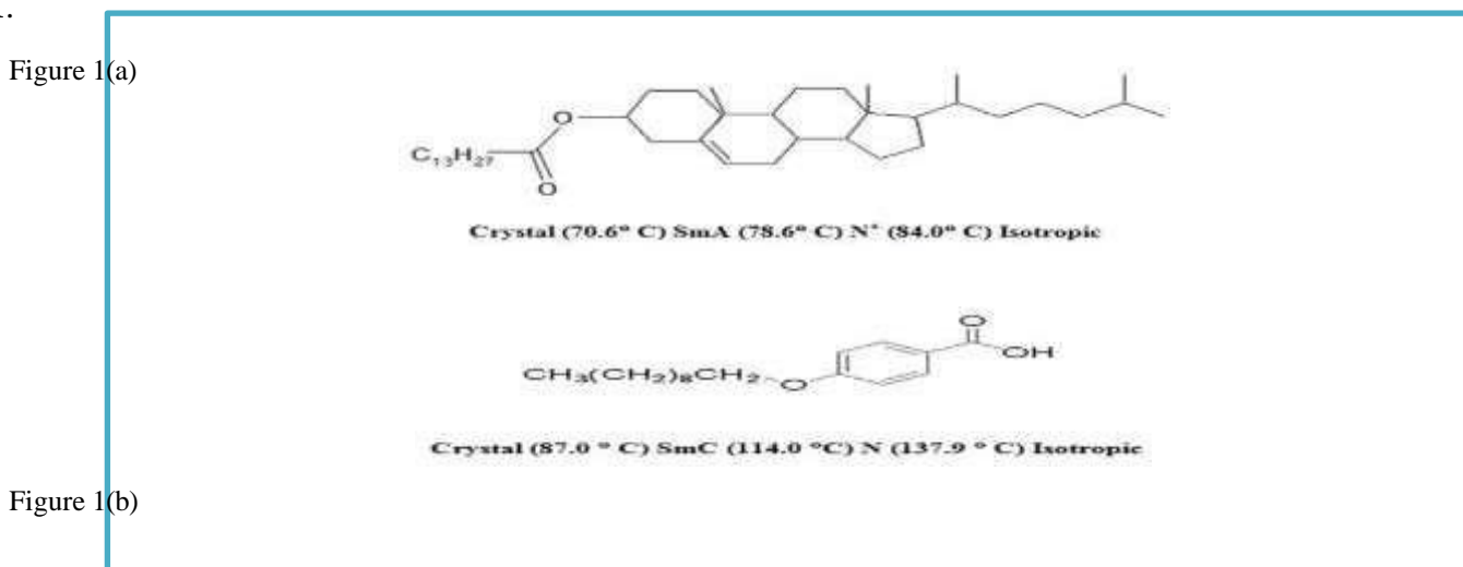
Figure 1: Chemical structures and phase transition temperatures of the liquid crystal materials (a) cholesteryl myristate (ChM) and (b) 4- n -decyloxy benzoic acid (DOBA) used for the preparation of the mixtures.
