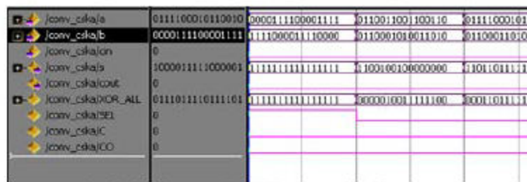
Figure 6: waveform of CONV-CSKA
