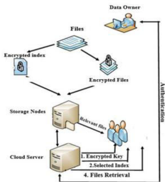
Fig. 1. Traditional Encrypted Search Architecture
