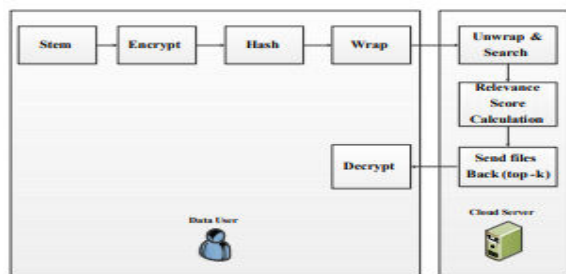
Fig. 2. ORS: Novel Process of Search and Retrieval
