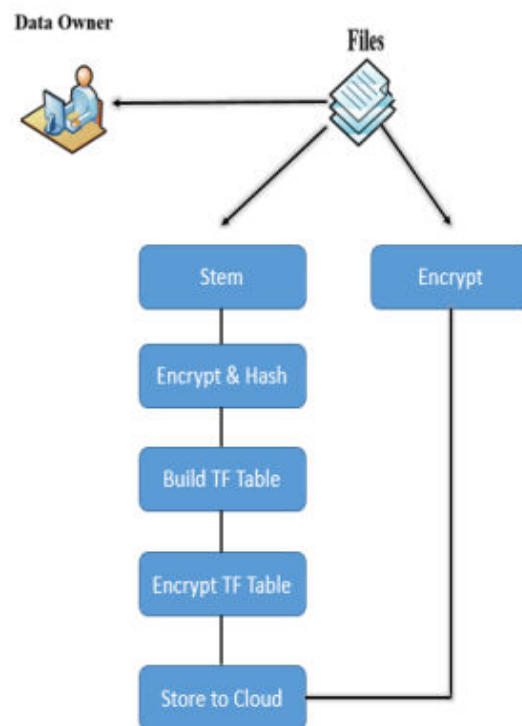
Fig 3. Process of Preprocessing and Indexing
