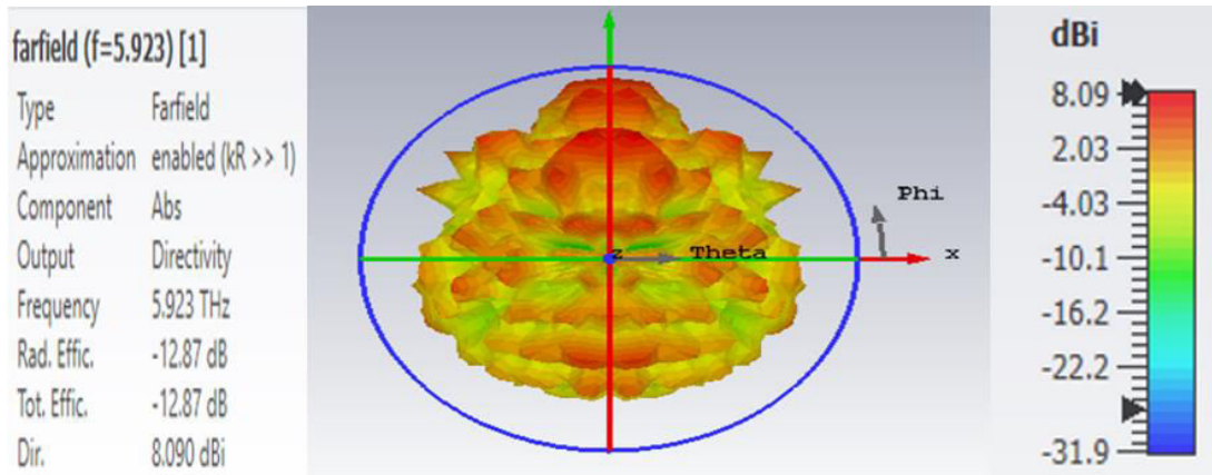
Figure. 20. Directivity at f = 5.923 is 8.090\text{dBi}
