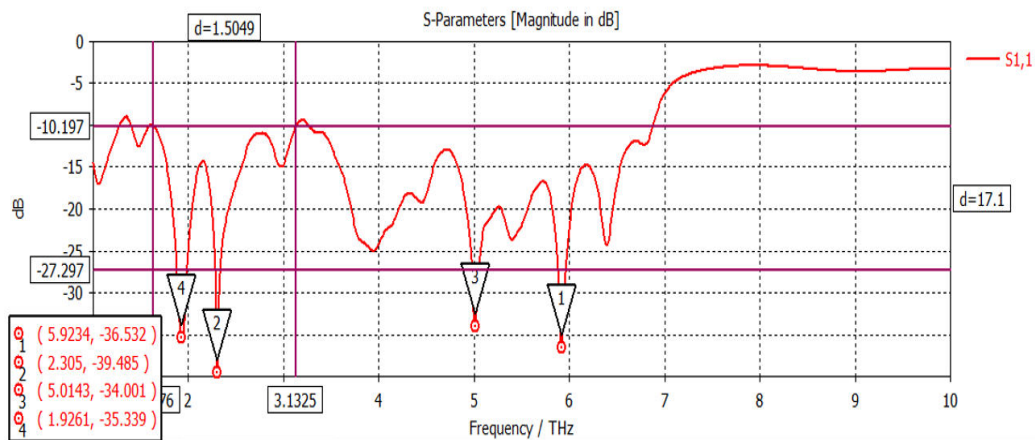
Figure. 13. Bandwidth at f = 2.305 is 1.5049 THz
