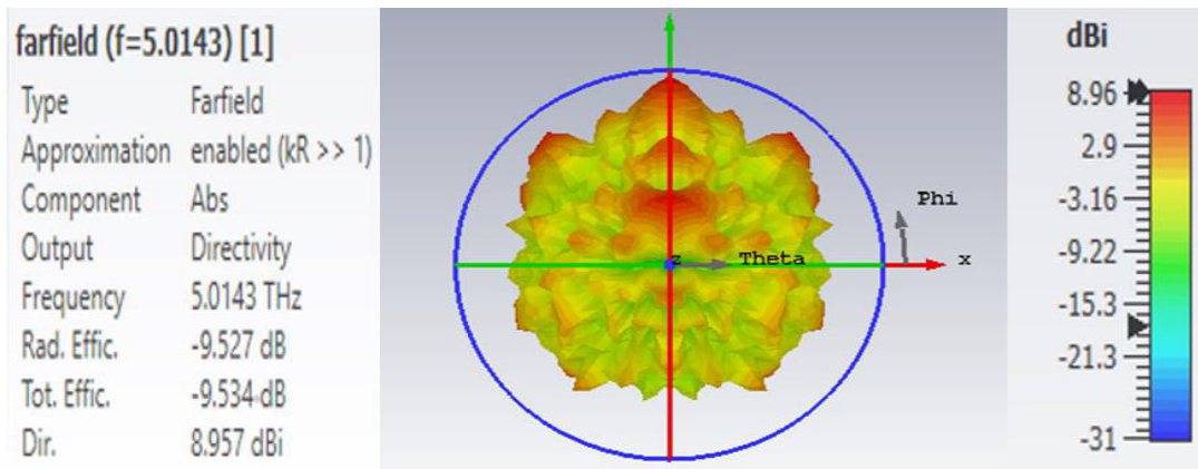
Figure. 19. Directivity at f = 5.0143 is 8.957\text{dBi}
