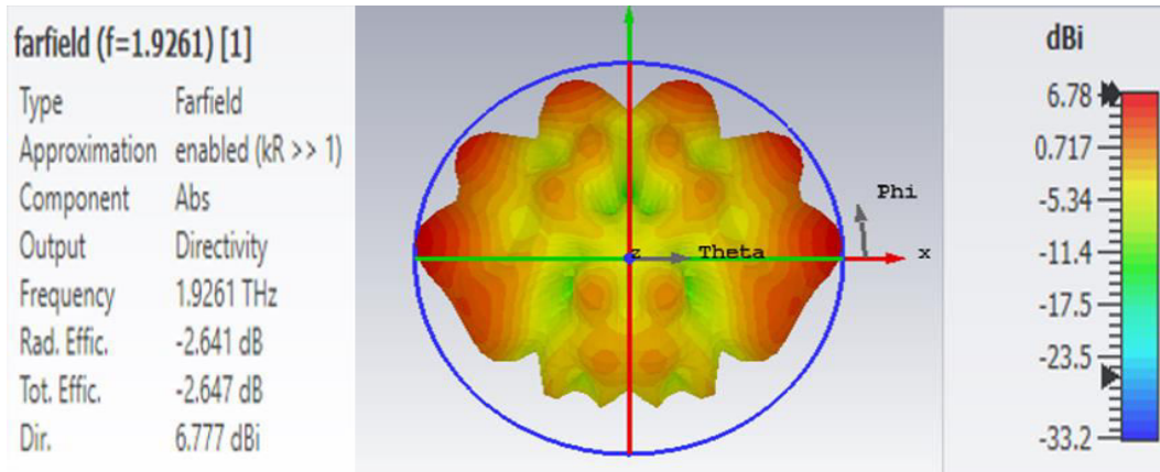
Figure. 17. Directivity at f = 1.9261 is 6.777dBi
