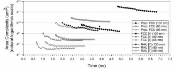
Fig. 5. Area-time diagram of FCUs.
