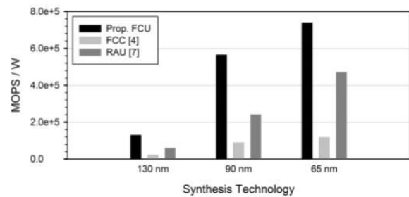
Fig. 6. MOPS/W values of FCUs at the lowest achievable clock periods
