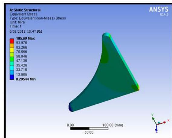
Fig.4.3. Stress model.
