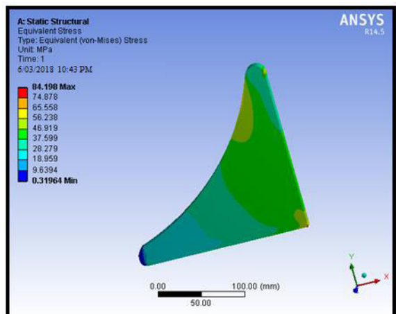
Fig.4.1. Strain model.
