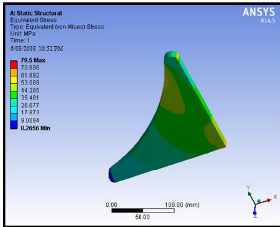
Fig.4.5. Stress model.
