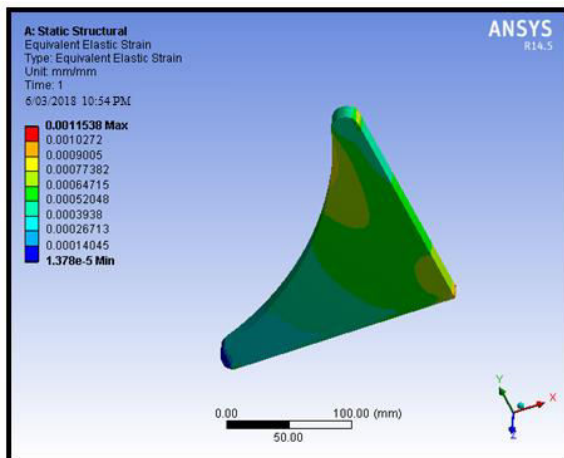
Fig.4.6. Strain model.
