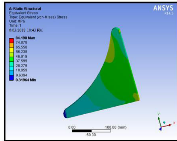
Fig.4.2. Stress model.
