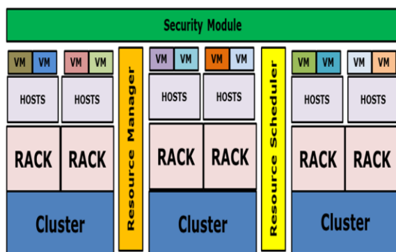
Fig. 1 Framework for Multipurpose Cloud Based Data Centre Network Security
