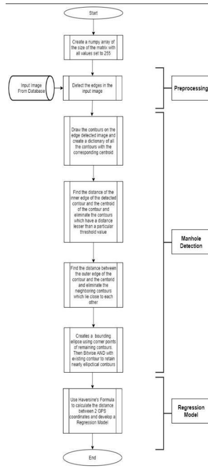
Fig. 1. Flowchart of the Proposed Methodology
