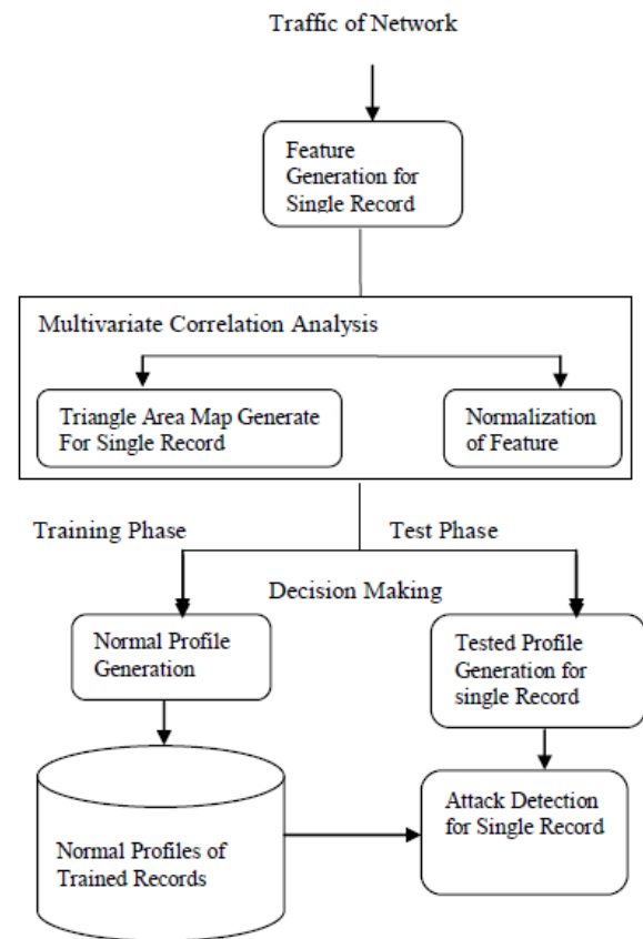
Figure 2. Framework of Denial of Service Attack Detection System
