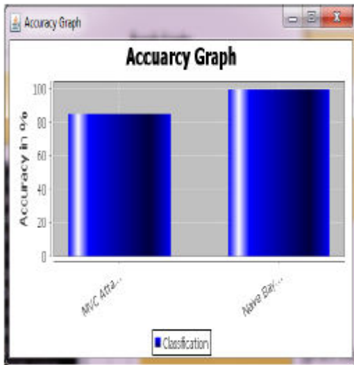
Figure 3. Accuracy Graph
