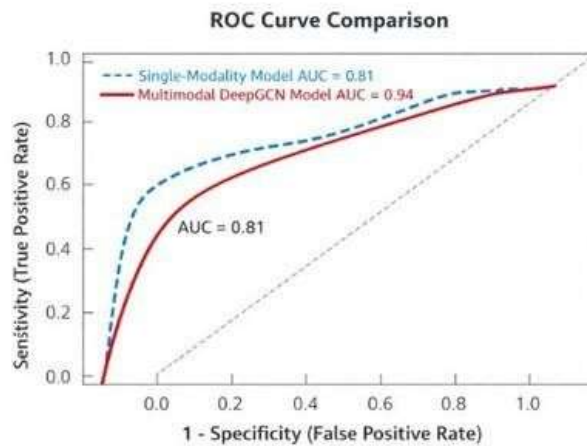
FIG 2.Roc Curve Graph
