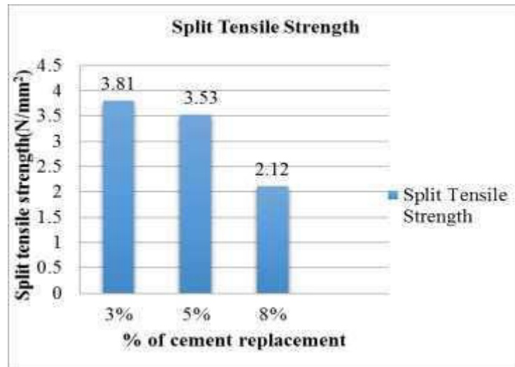
Fig. 6: Split Tensile Strength of Cylinder
