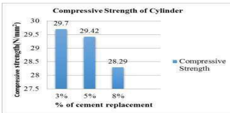
Fig. 5: Compressive Strength of Cylinder
