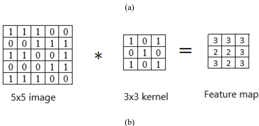
Figure 3: Example of convolution layer process (a) an image with size 5×5 is convolving with 3×3 kernel (b) Convolved feature map.
