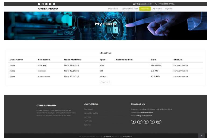
Fig 4:My Files
