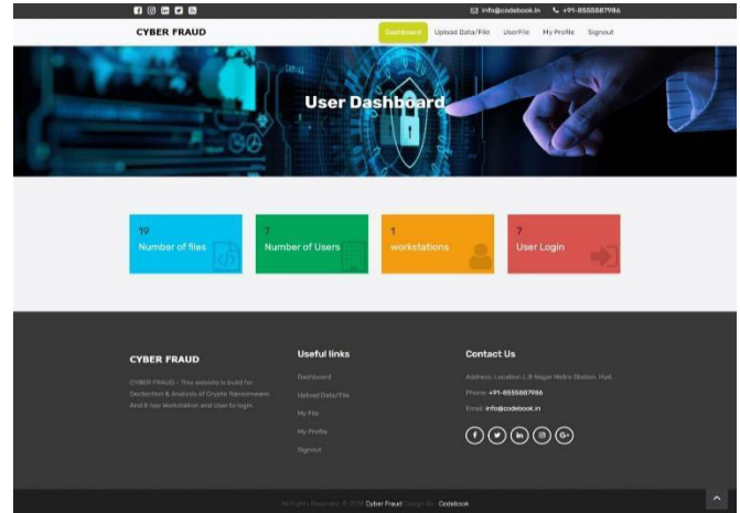
Fig2 :User Dashboard
