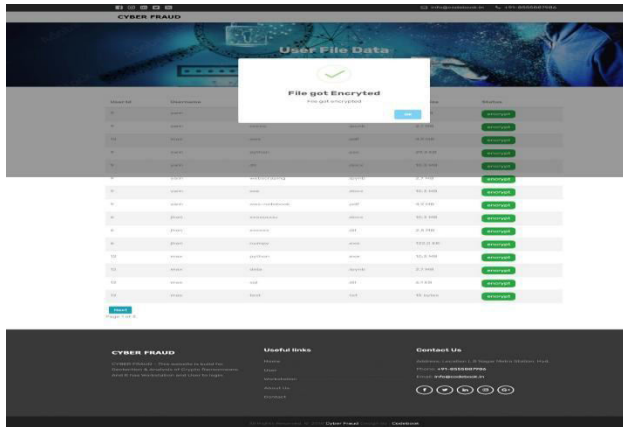
Fig5:Encrypted Files
