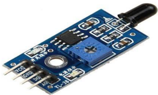
Fig flame-sensor
