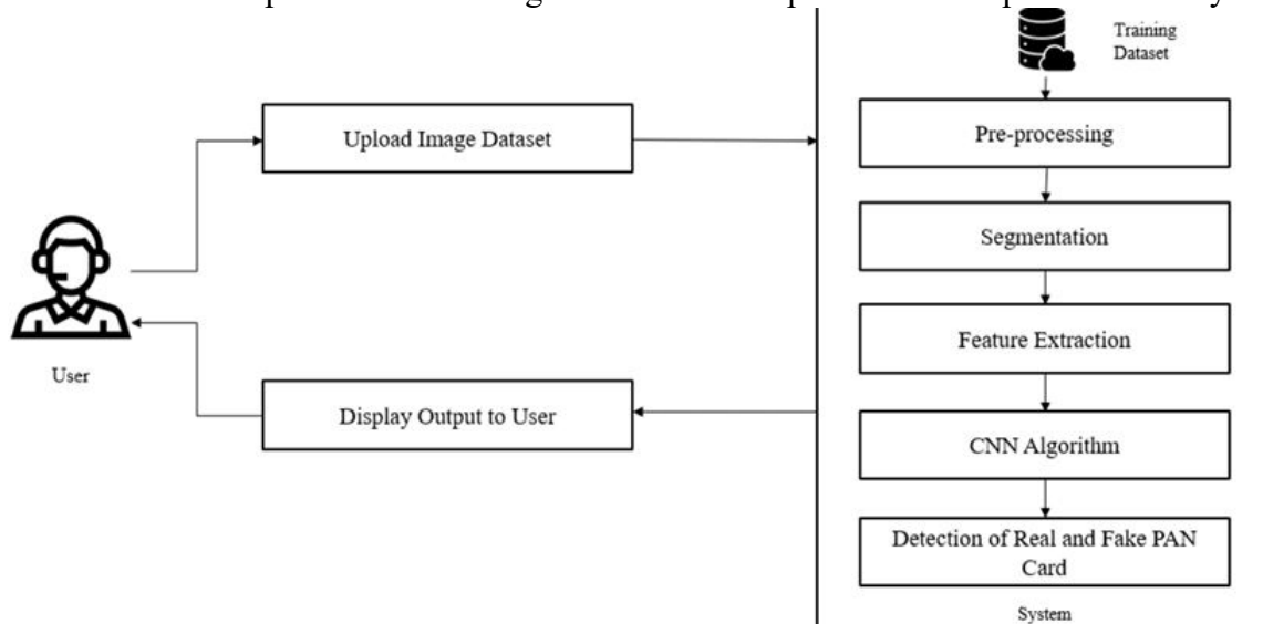
Fig1 PAN Card Tampering Detection system Architecture
