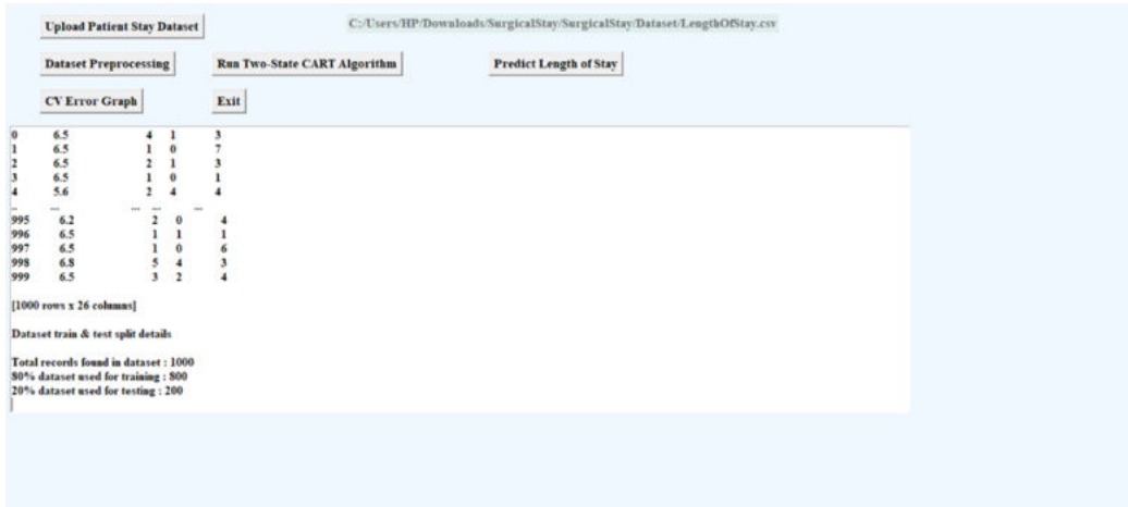
Figure 4: Preprocess Dataset
