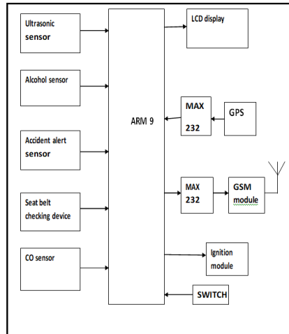
Fig.2: Block diagram
